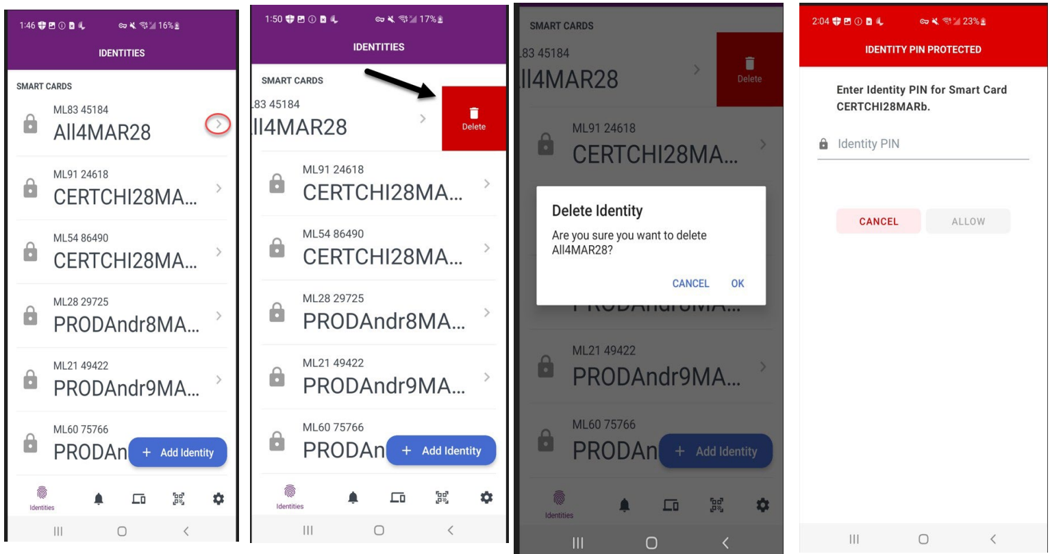
Figure 7: Deletion of Entrust Smart Credential Identity on an Android and Apple Device
